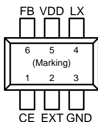
Figure1. Pin Assignment of FP6733
