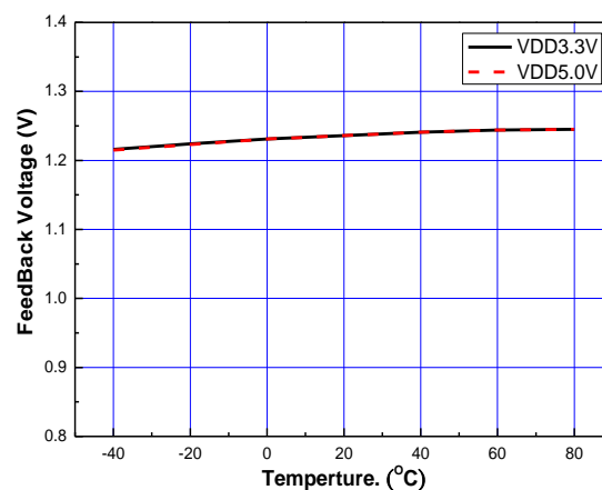
Figure 15. Temperature vs. Feedback Voltage 3.3Vi to 4LEDs (PWM control)
