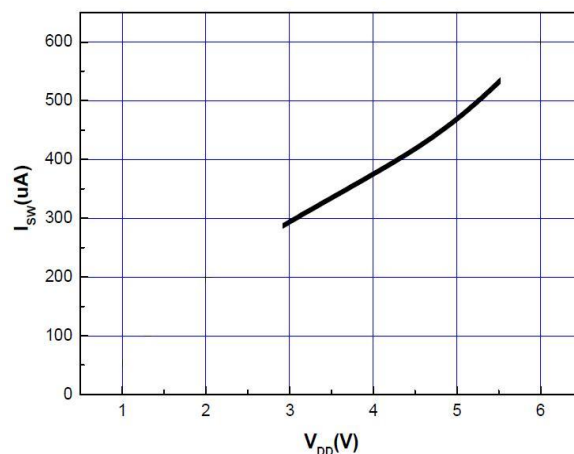
Figure 9. Operation Voltage vs. Switch Current
