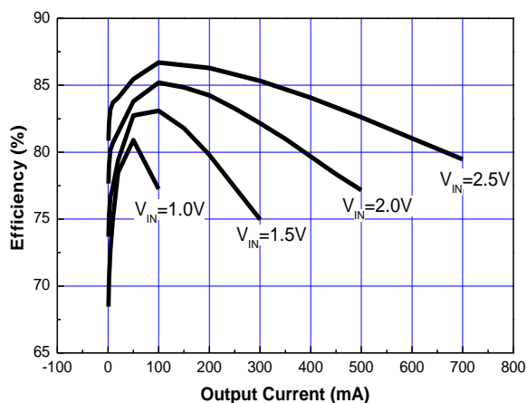
Figure 16. Efficiency ( V_{OUT}=3.3V )
