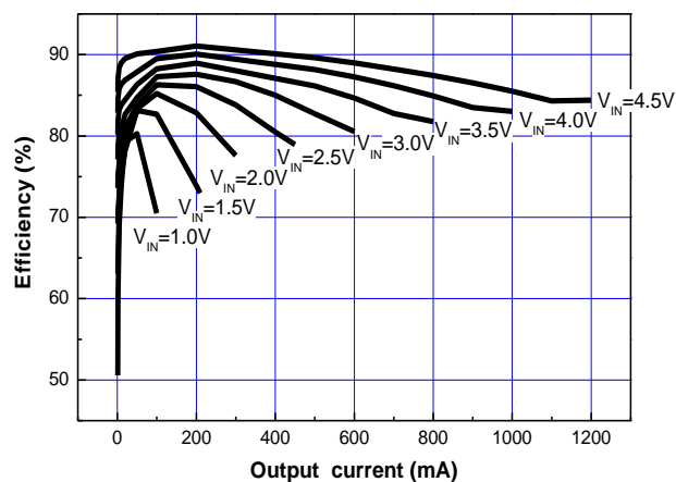
Figure 17. Efficiency ( V_{OUT}=5.0V ) (analog control)
