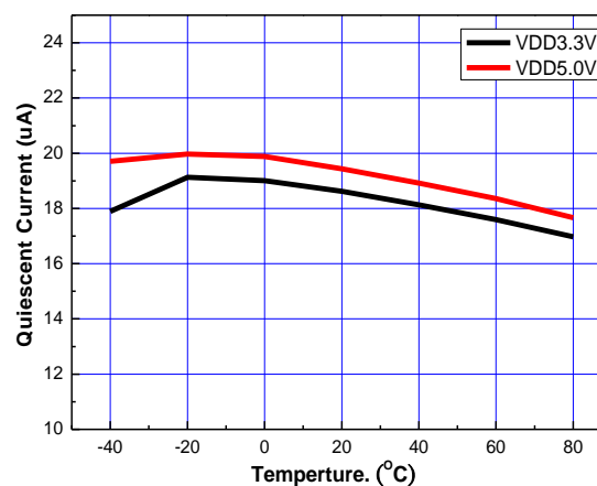
Figure 13. Temperature vs. Quiescent Current Vin=5V, 3LEDs, ILED=100mA, Cout=1μF
