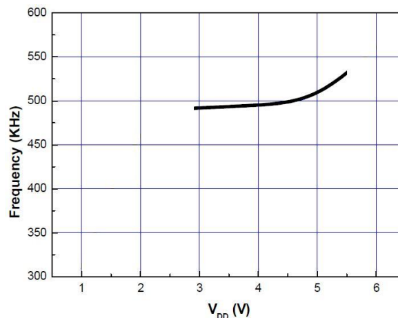
Figure 11. Operation Voltage vs. Frequency (analog control)
